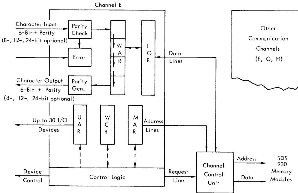
Figure 4-2. XDS 930 Direct Access Communication Channel, Block Diagram
