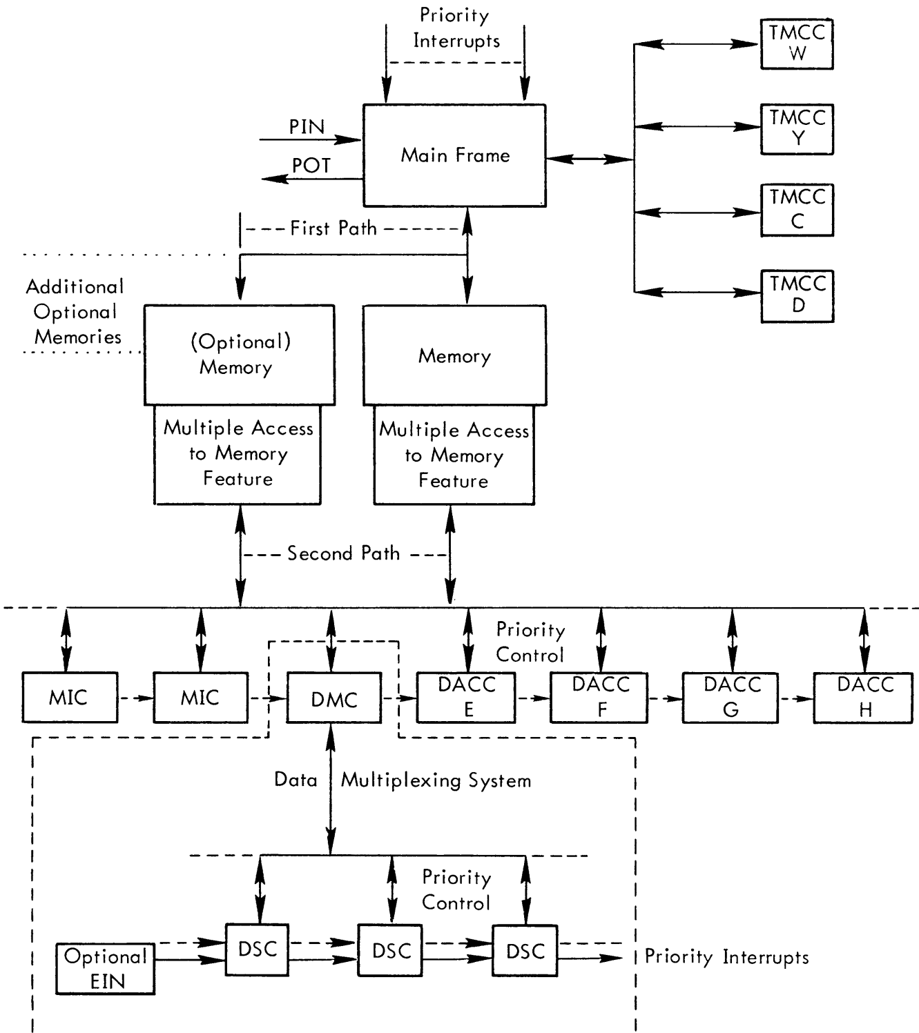
Figure A-1. XDS 930 Overall Computer Configuration
