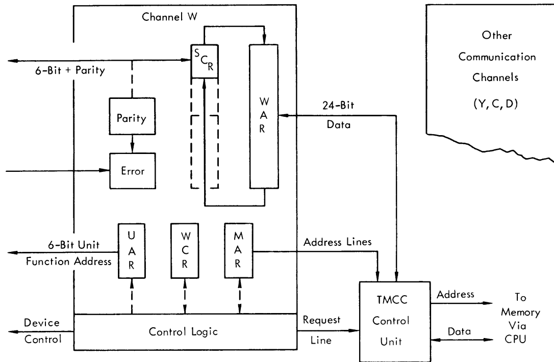
Figure 4-1. XDS 930 Time-Multiplexed Communication Channel, Block Diagram
